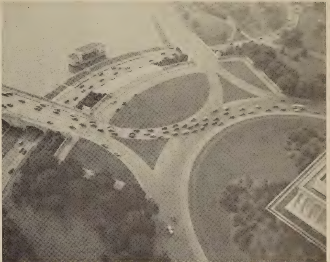
A portion of a traffic circle, showing weaving sections. Rerouting of traffic on some of the approaches to this circle has been resorted to as a means of reducing the conflicting cross movement at this point.
